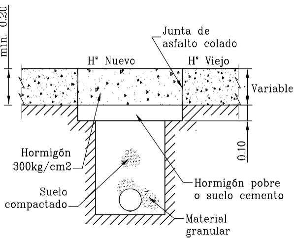
(c) TAPADA
