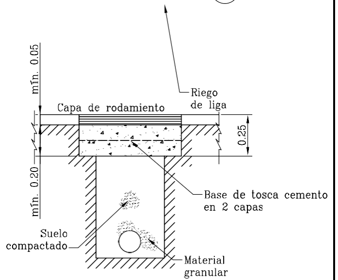
(c) TAPADA
